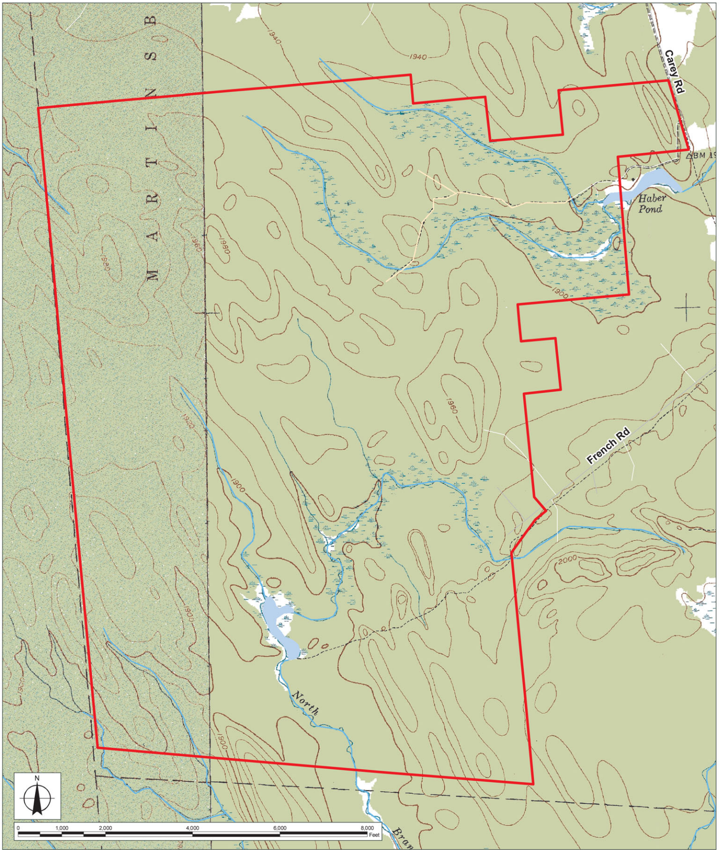
Figure 2: USGS Site Topography
