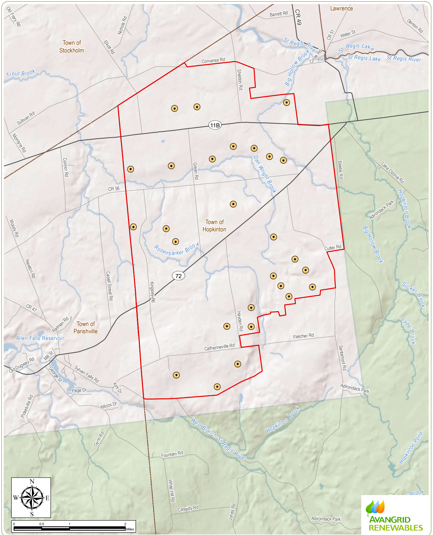
Figure 1. Preliminary Facility Layout
